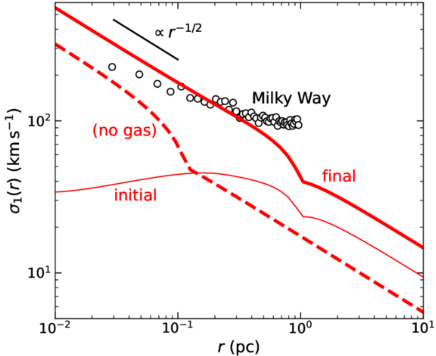
Figure 3. from Konstantinos Kritos and Joseph Silk 2026 Astrophys. J. 1004 doi:10.3847/1538-4357/ae731c https://dx.doi.org/10.3847/1538-4357/ae731c © 2026. The Author(s). Published by the American Astronomical Society.
