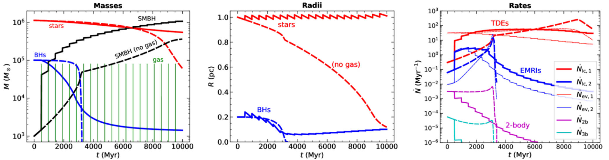
Figure 2. from Konstantinos Kritos and Joseph Silk 2026 Astrophys. J. 1004 doi:10.3847/1538-4357/ae731c https://dx.doi.org/10.3847/1538-4357/ae731c © 2026. The Author(s). Published by the American Astronomical Society.
