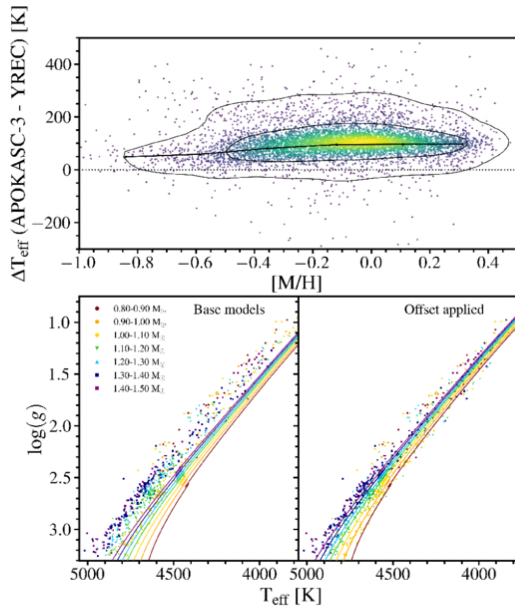
Figure 8. from Marc H. Pinsonneault et al 2026 Astrophys. J. 1006 doi:10.3847/1538-4357/ae71cf https://dx.doi.org/10.3847/1538-4357/ae71cf © 2026. The Author(s). Published by the American Astronomical Society.
