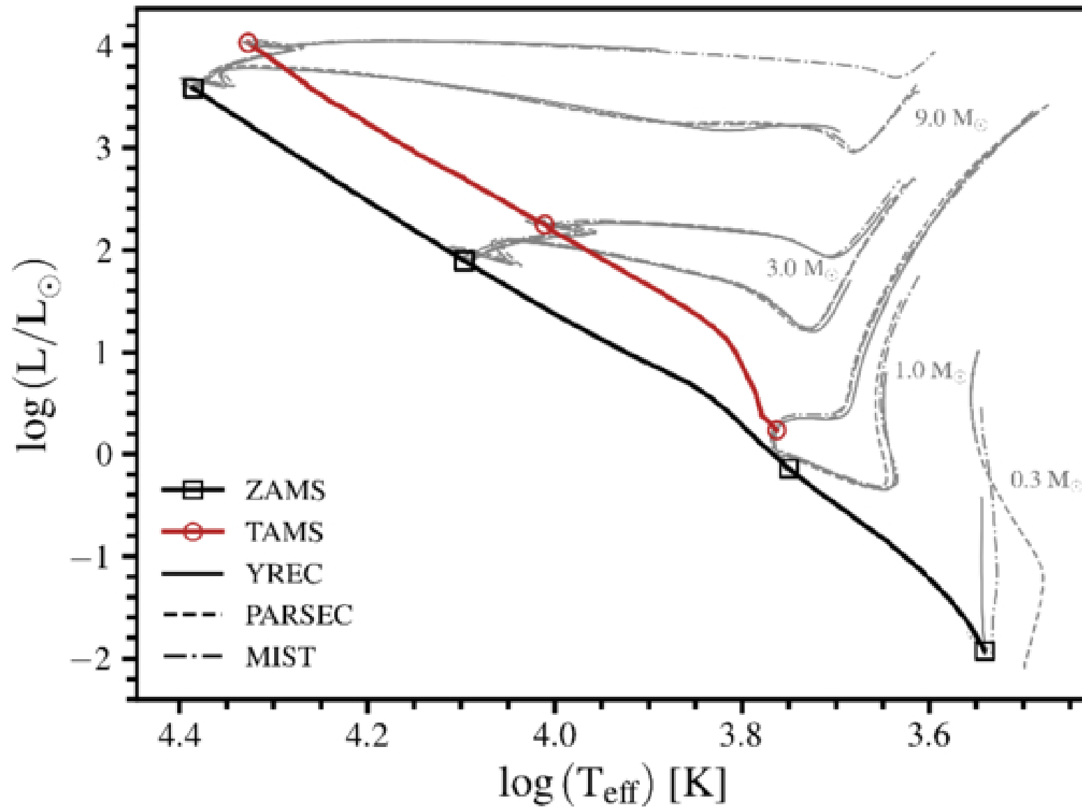
Figure 6. from Marc H. Pinsonneault et al 2026 Astrophys. J. 1006 doi:10.3847/1538-4357/ae71cf https://dx.doi.org/10.3847/1538-4357/ae71cf © 2026. The Author(s). Published by the American Astronomical Society.
