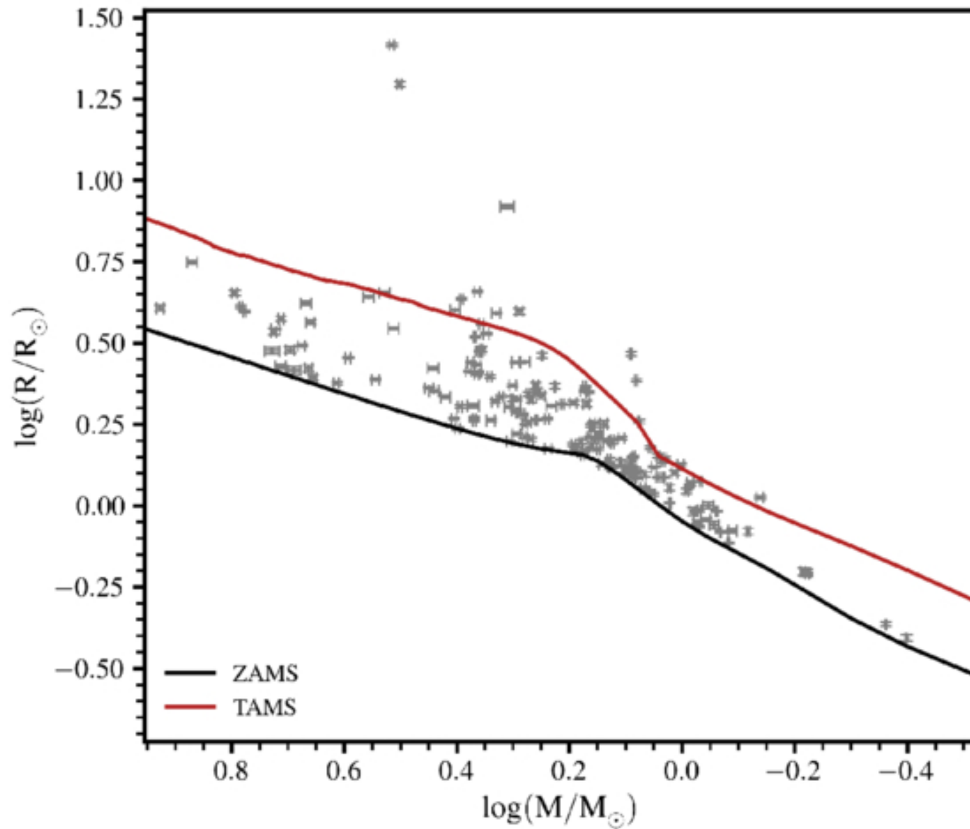
Figure 5. from Marc H. Pinsonneault et al 2026 Astrophys. J. 1006 doi:10.3847/1538-4357/ae71cf https://dx.doi.org/10.3847/1538-4357/ae71cf © 2026. The Author(s). Published by the American Astronomical Society.
