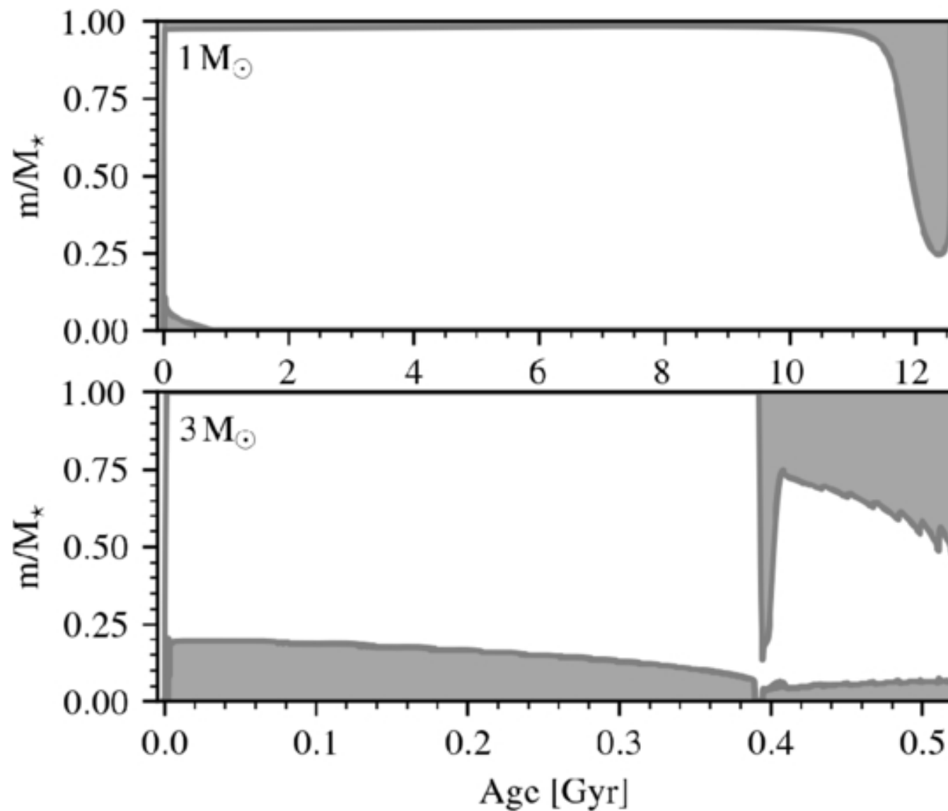
Figure 4. from Marc H. Pinsonneault et al 2026 Astrophys. J. 1006 doi:10.3847/1538-4357/ae71cf https://dx.doi.org/10.3847/1538-4357/ae71cf © 2026. The Author(s). Published by the American Astronomical Society.
