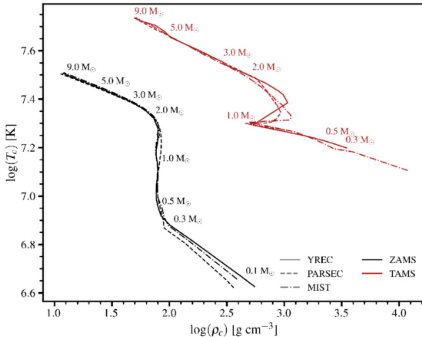
Figure 3. from Marc H. Pinsonneault et al 2026 Astrophys. J. 1006 doi:10.3847/1538-4357/ae71cf https://dx.doi.org/10.3847/1538-4357/ae71cf © 2026. The Author(s). Published by the American Astronomical Society.
