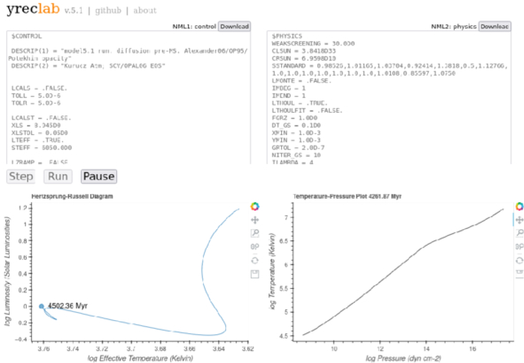
Figure 21. from Marc H. Pinsonneault et al 2026 Astrophys. J. 1006 doi:10.3847/1538-4357/ae71cf https://dx.doi.org/10.3847/1538-4357/ae71cf © 2026. The Author(s). Published by the American Astronomical Society.
