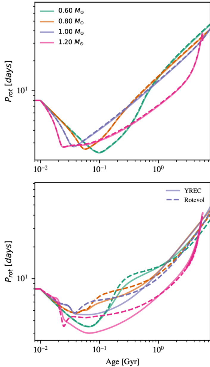
Figure 19. from Marc H. Pinsonneault et al 2026 Astrophys. J. 1006 doi:10.3847/1538-4357/ae71cf https://dx.doi.org/10.3847/1538-4357/ae71cf © 2026. The Author(s). Published by the American Astronomical Society.
