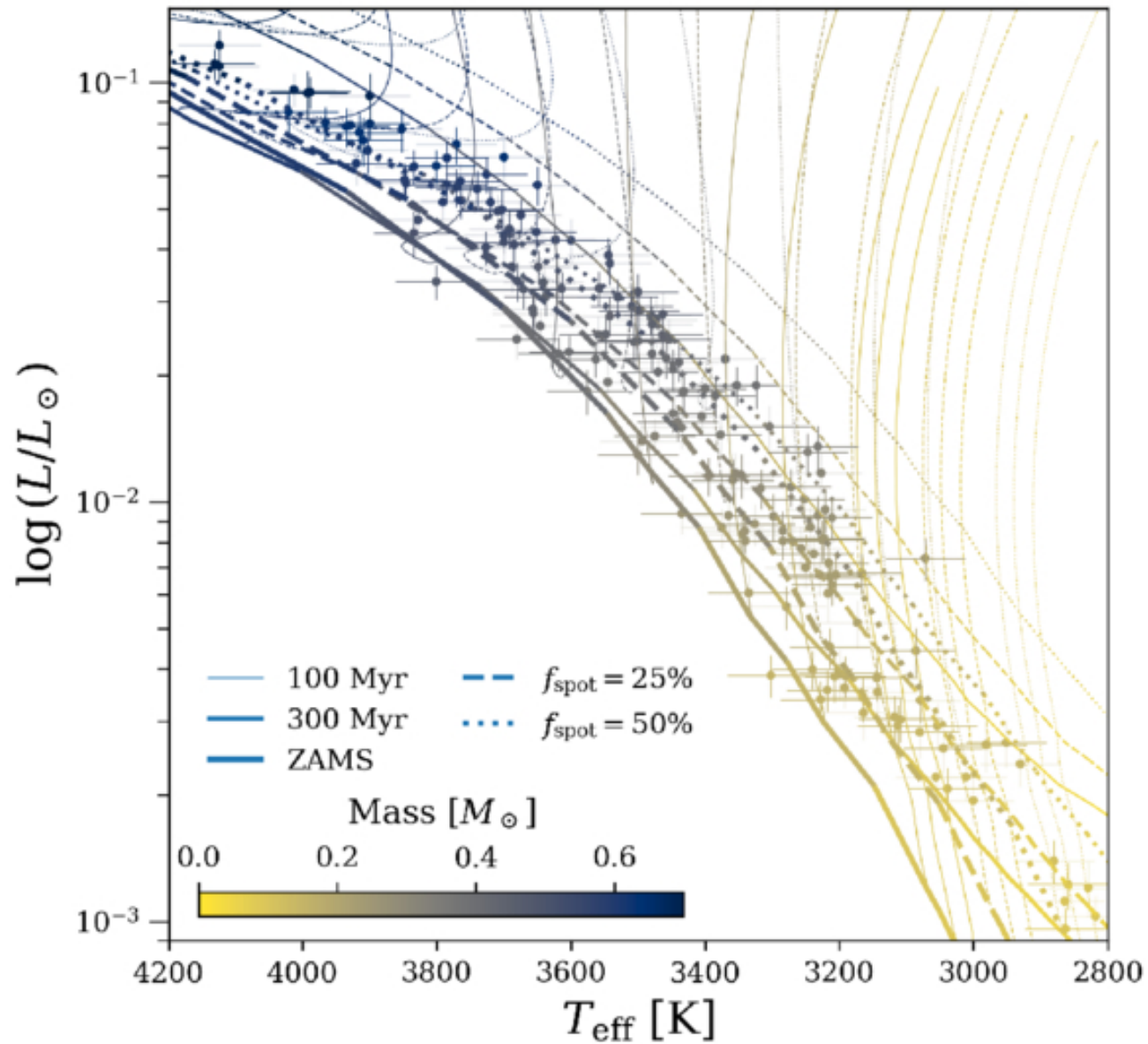
Figure 16. from Marc H. Pinsonneault et al 2026 Astrophys. J. 1006 doi:10.3847/1538-4357/ae71cf https://dx.doi.org/10.3847/1538-4357/ae71cf © 2026. The Author(s). Published by the American Astronomical Society.
