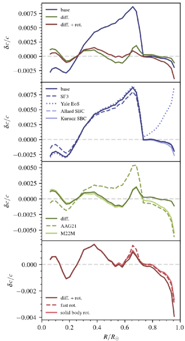
Figure 12. from Marc H. Pinsonneault et al 2026 Astrophys. J. 1006 doi:10.3847/1538-4357/ae71cf https://dx.doi.org/10.3847/1538-4357/ae71cf © 2026. The Author(s). Published by the American Astronomical Society.
