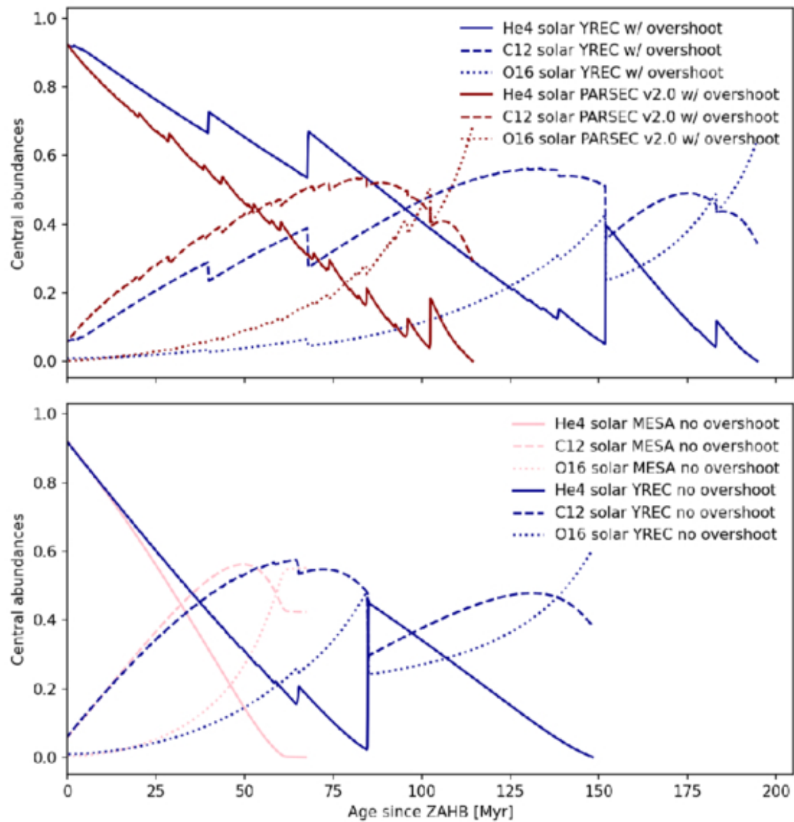
Figure 11. from Marc H. Pinsonneault et al 2026 Astrophys. J. 1006 doi:10.3847/1538-4357/ae71cf https://dx.doi.org/10.3847/1538-4357/ae71cf © 2026. The Author(s). Published by the American Astronomical Society.
