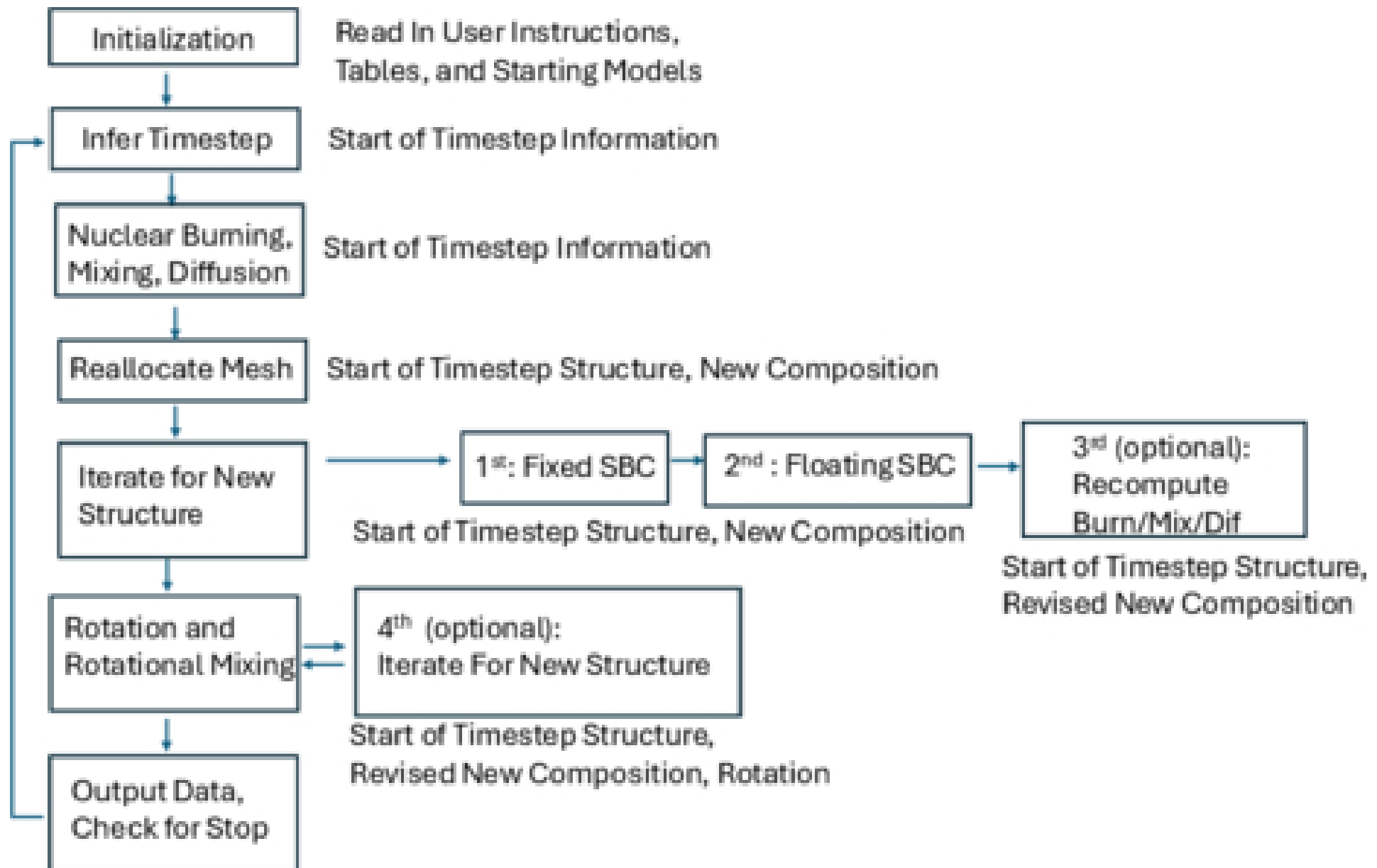
Figure 1. from Marc H. Pinsonneault et al 2026 Astrophys. J. 1006 doi:10.3847/1538-4357/ae71cf https://dx.doi.org/10.3847/1538-4357/ae71cf © 2026. The Author(s). Published by the American Astronomical Society.
