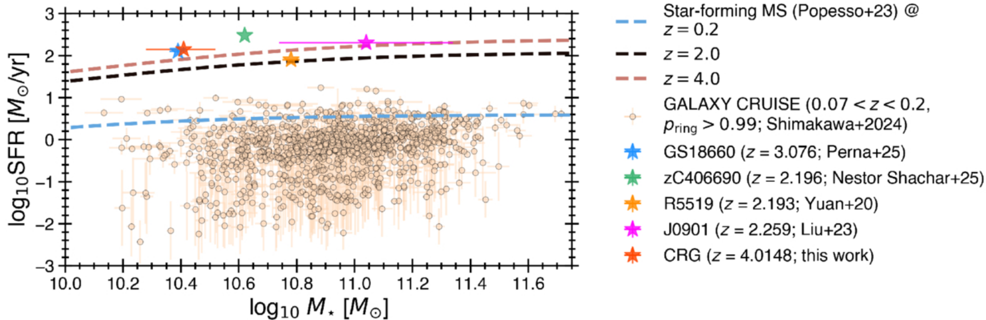
Figure 6. from David Vizgan et al 2026 Astrophys. J. 1004 doi:10.3847/1538-4357/ae7103 https://dx.doi.org/10.3847/1538-4357/ae7103 © 2026. The Author(s). Published by the American Astronomical Society.
