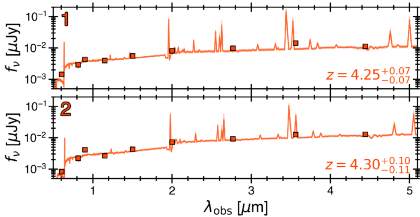
Figure 4. from David Vizgan et al 2026 Astrophys. J. 1004 doi:10.3847/1538-4357/ae7103 https://dx.doi.org/10.3847/1538-4357/ae7103 © 2026. The Author(s). Published by the American Astronomical Society.
