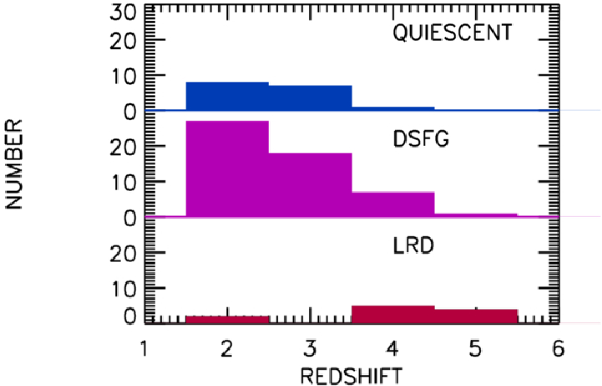
Figure 9. from A. J. Barger et al 2026 Astrophys. J. 1004 doi:10.3847/1538-4357/ae7101 https://dx.doi.org/10.3847/1538-4357/ae7101 © 2026. The Author(s). Published by the American Astronomical Society.
