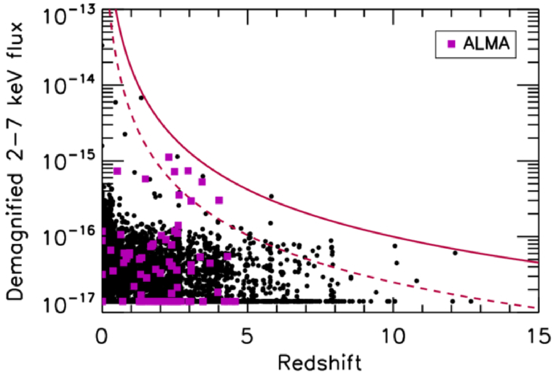
Figure 4. from A. J. Barger et al 2026 Astrophys. J. 1004 doi:10.3847/1538-4357/ae7101 https://dx.doi.org/10.3847/1538-4357/ae7101 © 2026. The Author(s). Published by the American Astronomical Society.
