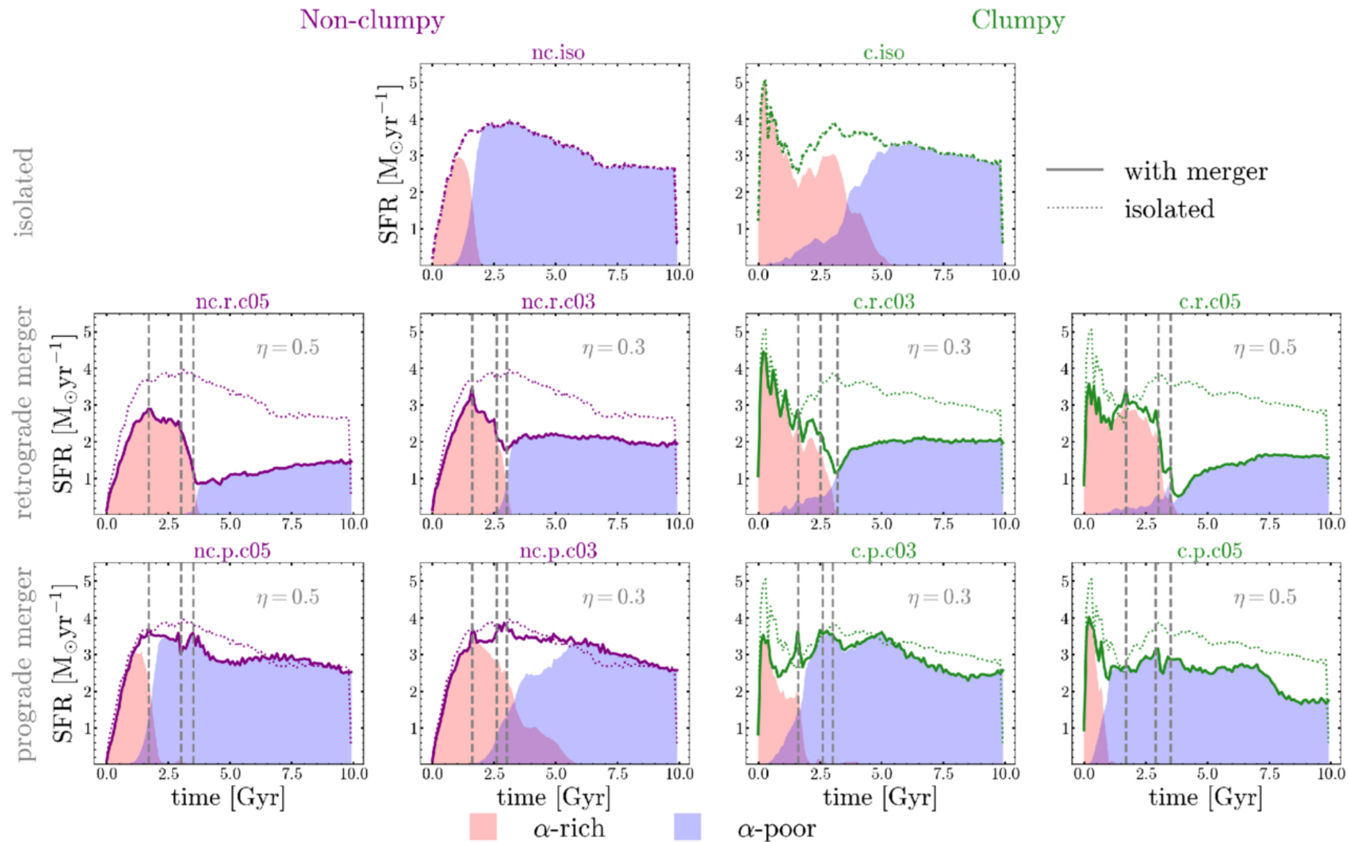
Figure 5. from João A. S. Amarante et al 2026 Astrophys. J. 1004 doi:10.3847/1538-4357/ae70fe https://dx.doi.org/10.3847/1538-4357/ae70fe © 2026. The Author(s). Published by the American Astronomical Society.
