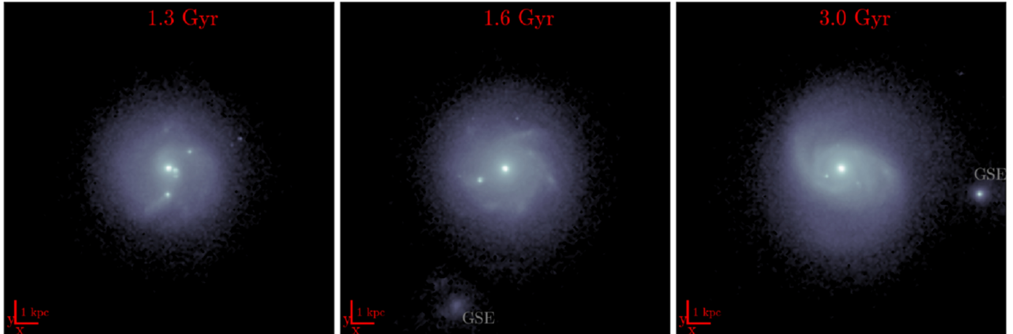
Figure 2. from João A. S. Amarante et al 2026 Astrophys. J. 1004 doi:10.3847/1538-4357/ae70fe https://dx.doi.org/10.3847/1538-4357/ae70fe © 2026. The Author(s). Published by the American Astronomical Society.
