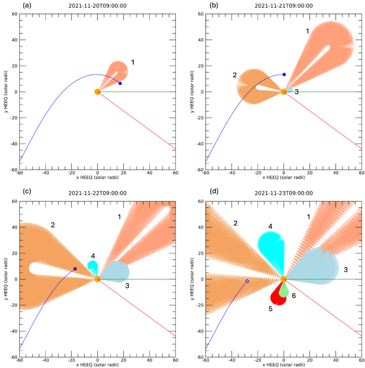
Figure 4. from Carlos R. Braga et al 2026 Astrophys. J. 1005 doi:10.3847/1538-4357/ae7084 https://dx.doi.org/10.3847/1538-4357/ae7084 © 2026. The Author(s). Published by the American Astronomical Society.
