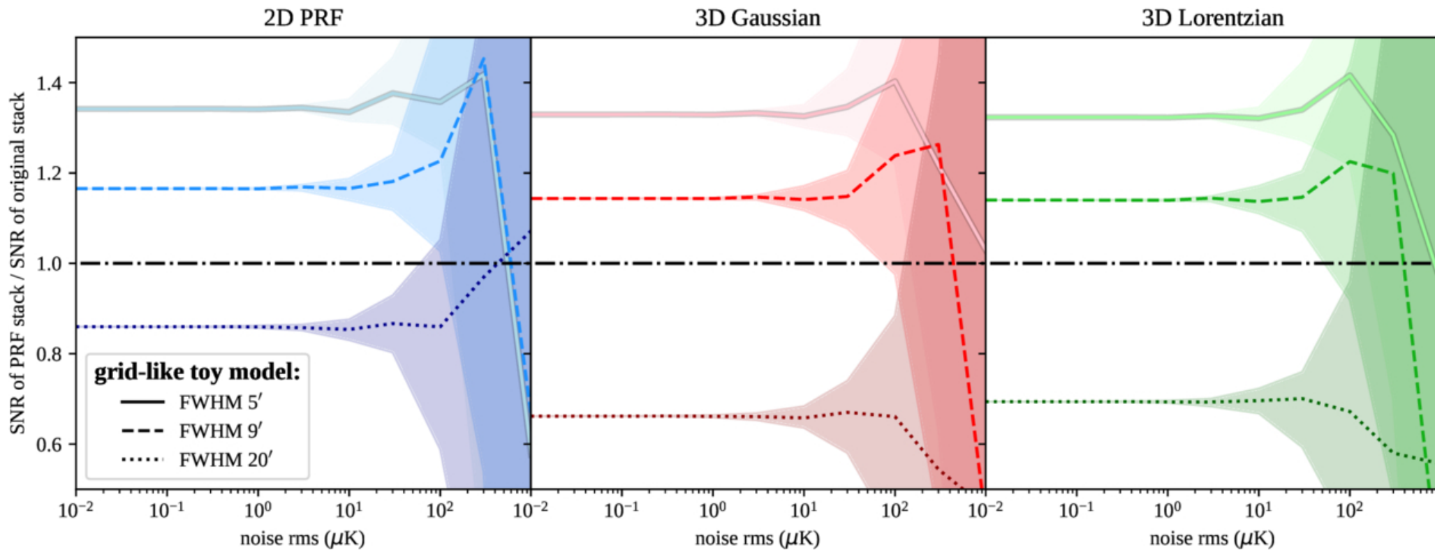
Figure 4. from Ella M. Mansfield et al 2026 Astrophys. J. 1005 doi:10.3847/1538-4357/ae7082 https://dx.doi.org/10.3847/1538-4357/ae7082 © 2026. The Author(s). Published by the American Astronomical Society.
