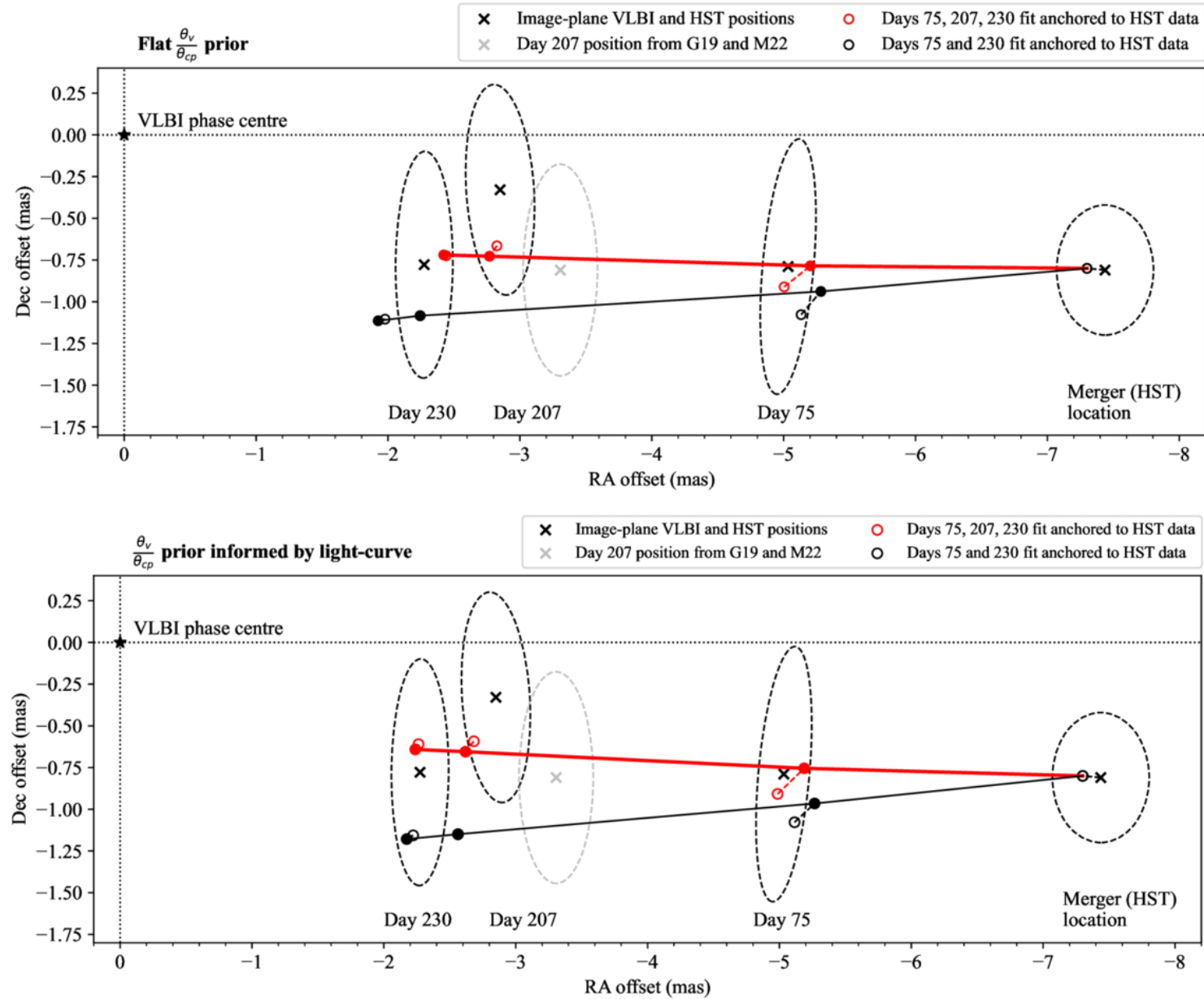
Figure 2. from Kelly Gourdji et al 2026 Astrophys. J. 1005 doi:10.3847/1538-4357/ae706c https://dx.doi.org/10.3847/1538-4357/ae706c © 2026. The Author(s). Published by the American Astronomical Society.
