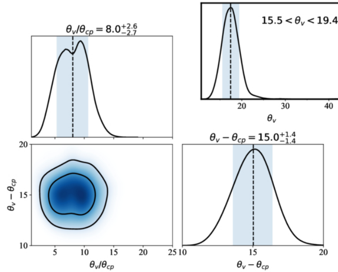
Panel D: days 0, 75, 207, 230; \frac{\theta_v}{\theta_{cp}} prior informed by light-curve
