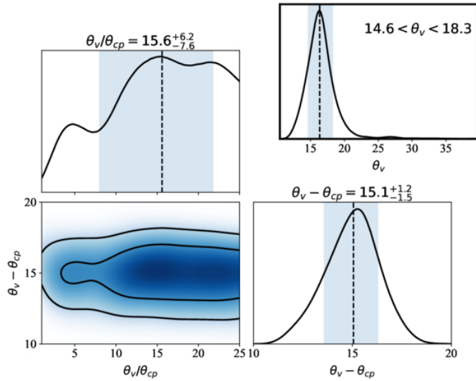
Panel C: days 0, 75, 207, 230; flat \frac{\theta_v}{\theta_{cp}} prior
