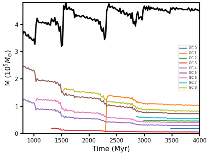
Figure 7. from Ismael Khan et al 2026 Astrophys. J. 1005 doi:10.3847/1538-4357/ae6fb7 https://dx.doi.org/10.3847/1538-4357/ae6fb7 © 2026. The Author(s). Published by the American Astronomical Society.
