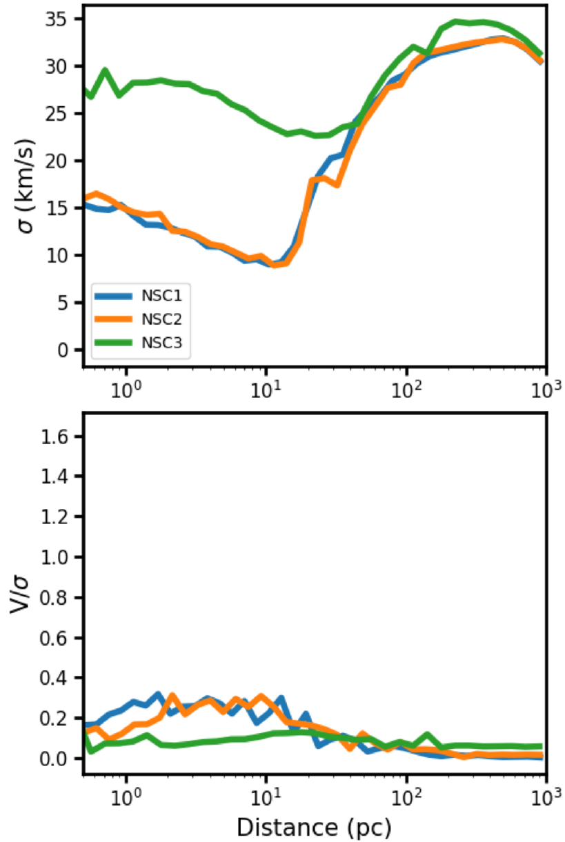
Figure 11. from Ismael Khan et al 2026 Astrophys. J. 1005 doi:10.3847/1538-4357/ae6fb7 https://dx.doi.org/10.3847/1538-4357/ae6fb7 © 2026. The Author(s). Published by the American Astronomical Society.
