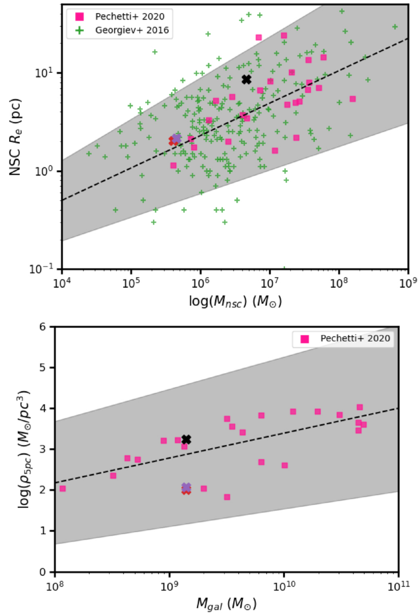
Figure 10. from Ismael Khan et al 2026 Astrophys. J. 1005 doi:10.3847/1538-4357/ae6fb7 https://dx.doi.org/10.3847/1538-4357/ae6fb7 © 2026. The Author(s). Published by the American Astronomical Society.
