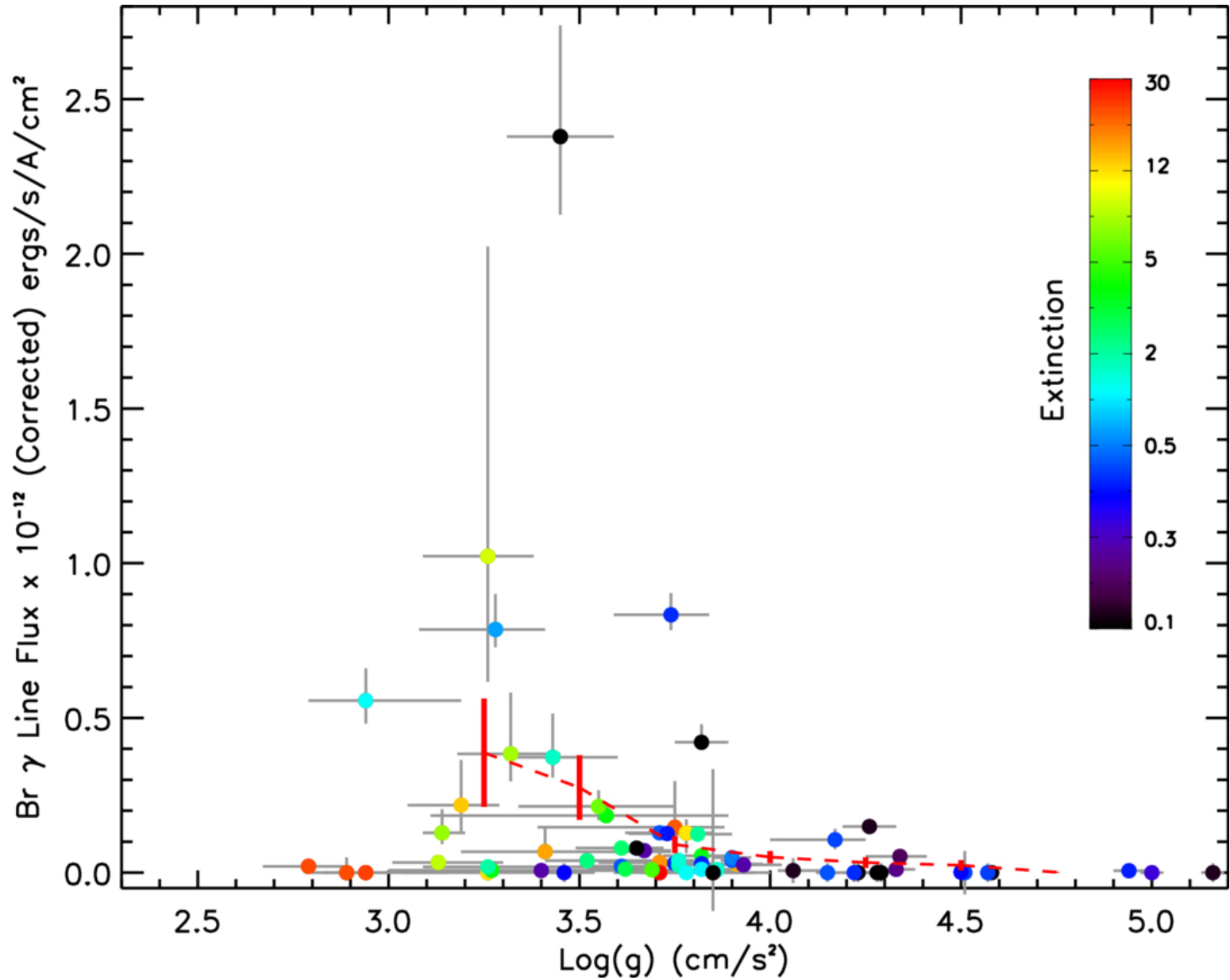
Figure 4. from Michael Connelley et al 2026 Astrophys. J. 1005 doi:10.3847/1538-4357/ae6fab https://dx.doi.org/10.3847/1538-4357/ae6fab © 2026. The Author(s). Published by the American Astronomical Society.
