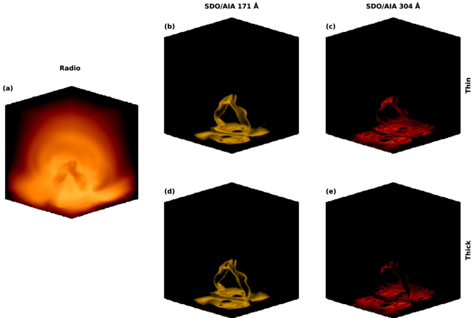
Figure 6. from Wentai Fu et al 2026 Astrophys. J. 1004 doi:10.3847/1538-4357/ae6f0d https://dx.doi.org/10.3847/1538-4357/ae6f0d © 2026. The Author(s). Published by the American Astronomical Society.
