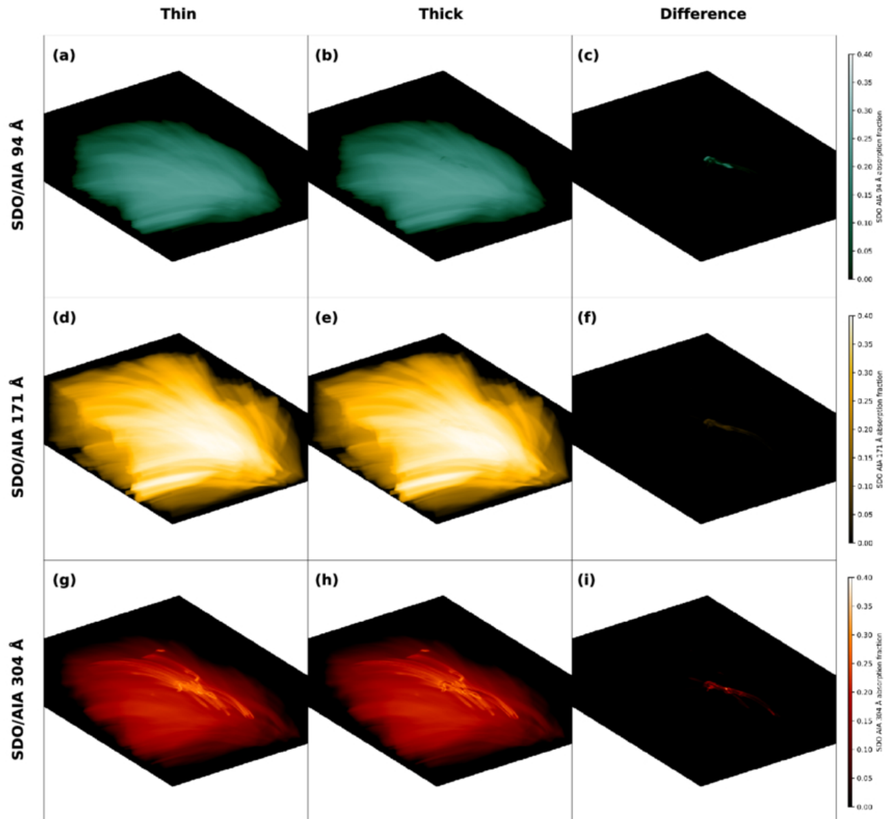
Figure 4. from Wentai Fu et al 2026 Astrophys. J. 1004 doi:10.3847/1538-4357/ae6f0d https://dx.doi.org/10.3847/1538-4357/ae6f0d © 2026. The Author(s). Published by the American Astronomical Society.
