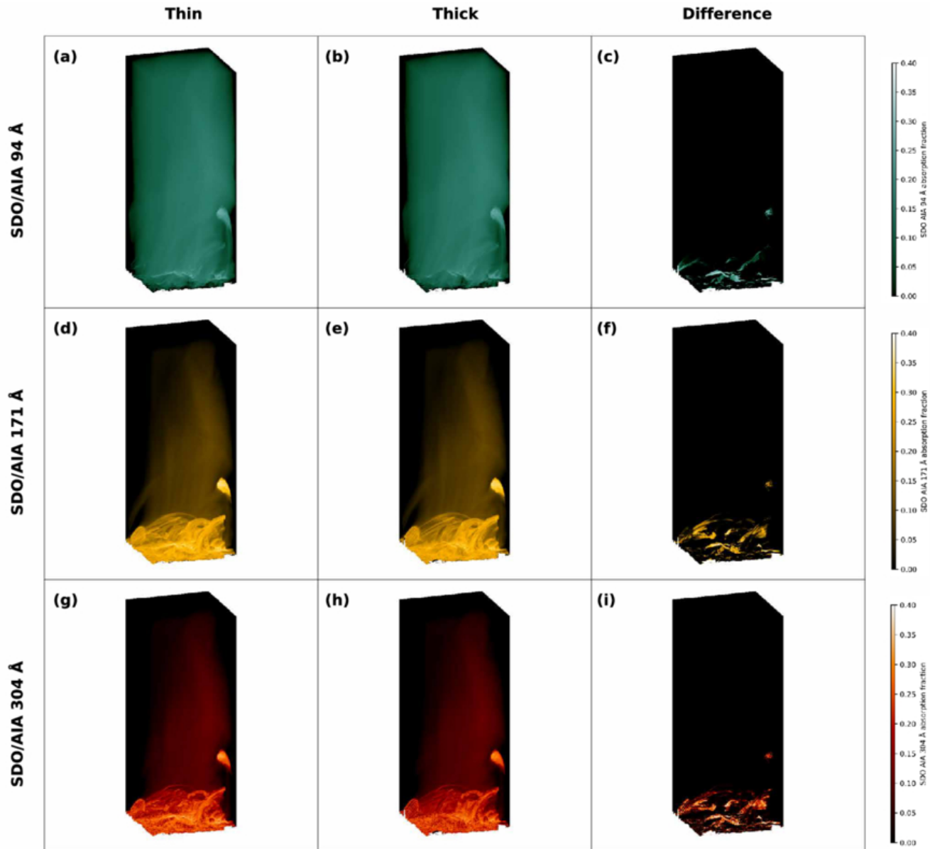
Figure 3. from Wentai Fu et al 2026 Astrophys. J. 1004 doi:10.3847/1538-4357/ae6f0d https://dx.doi.org/10.3847/1538-4357/ae6f0d © 2026. The Author(s). Published by the American Astronomical Society.
