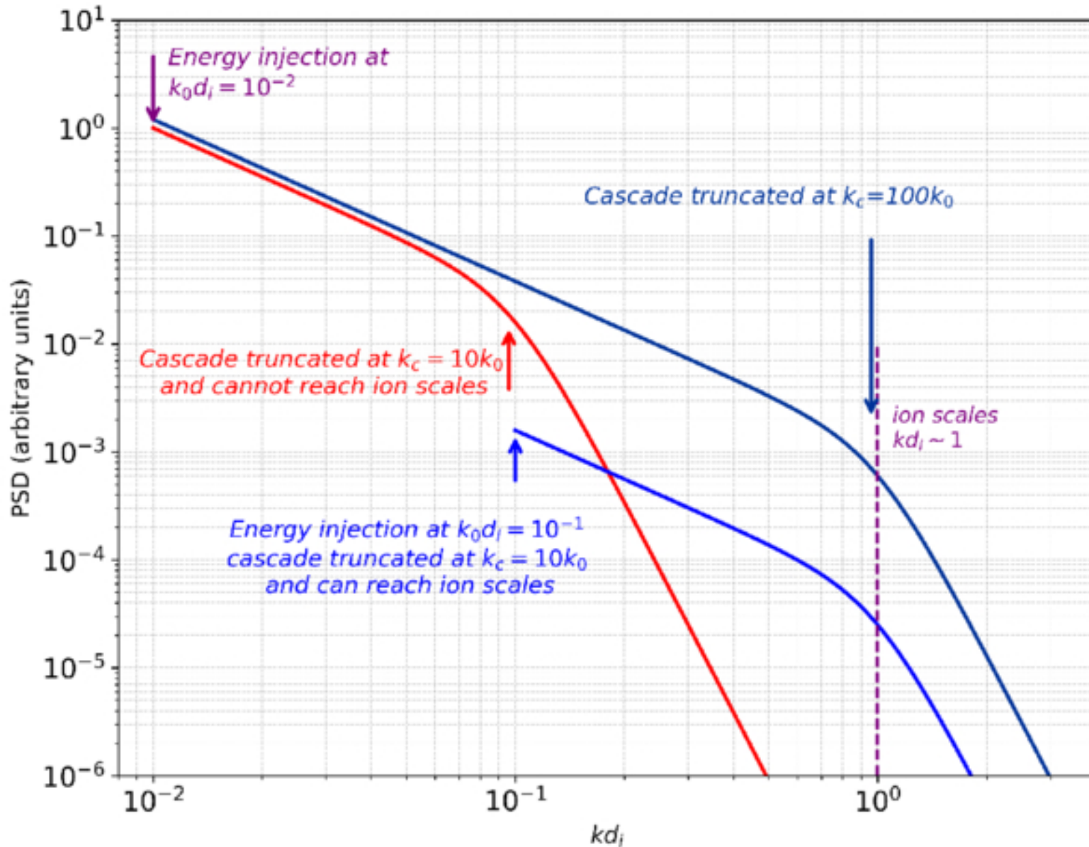
Figure 5. from Chuanpeng Hou et al 2026 Astrophys. J. 1004 doi:10.3847/1538-4357/ae6f0a https://dx.doi.org/10.3847/1538-4357/ae6f0a © 2026. The Author(s). Published by the American Astronomical Society.
