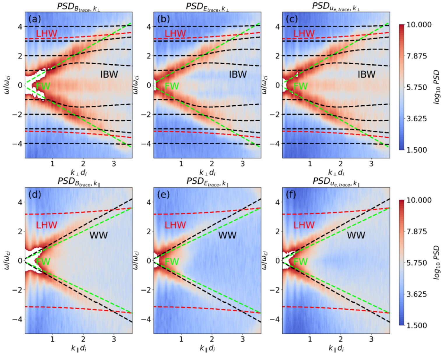
Figure 3. from Chuanpeng Hou et al 2026 Astrophys. J. 1004 doi:10.3847/1538-4357/ae6f0a https://dx.doi.org/10.3847/1538-4357/ae6f0a © 2026. The Author(s). Published by the American Astronomical Society.
