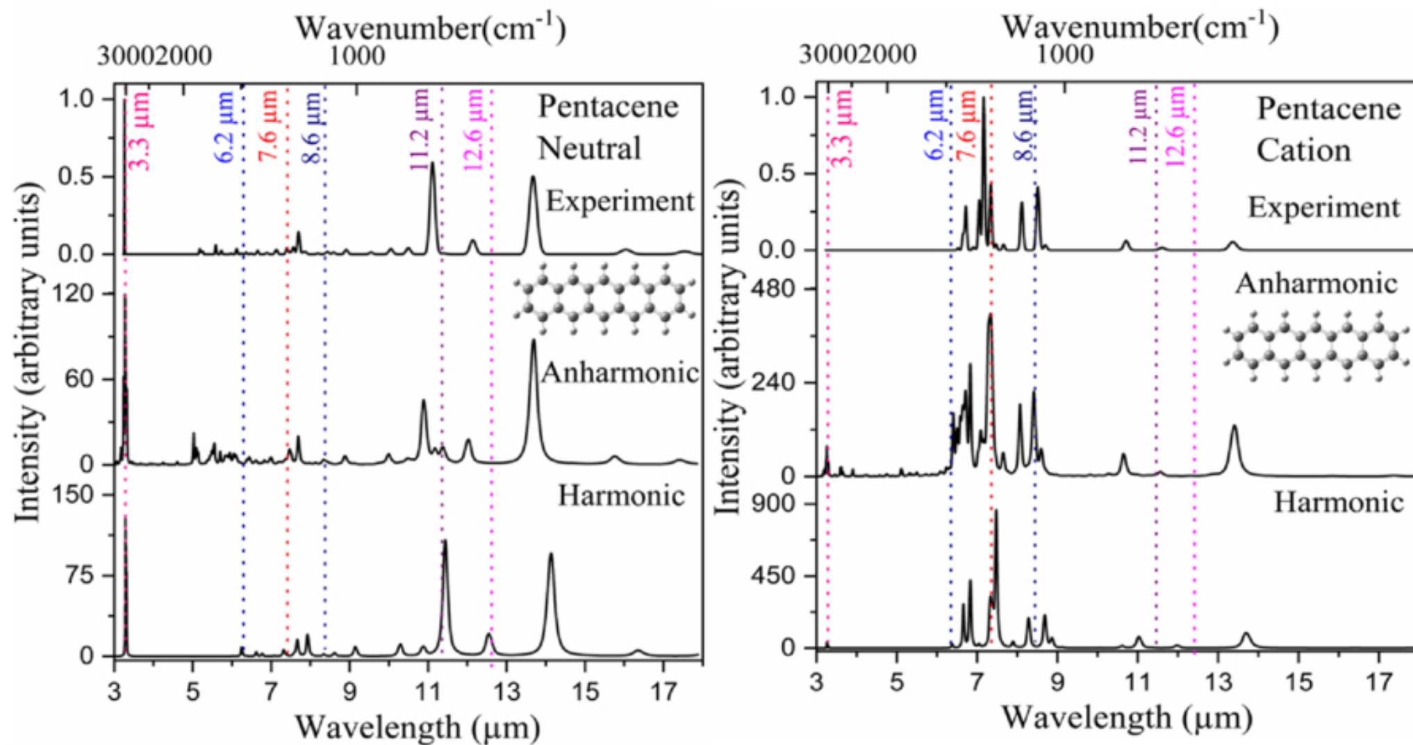
Figure 8. from Venkata Lakshmi Karri et al 2026 Astrophys. J. 1008 doi:10.3847/1538-4357/ae6eef https://dx.doi.org/10.3847/1538-4357/ae6eef © 2026. The Author(s). Published by the American Astronomical Society.
