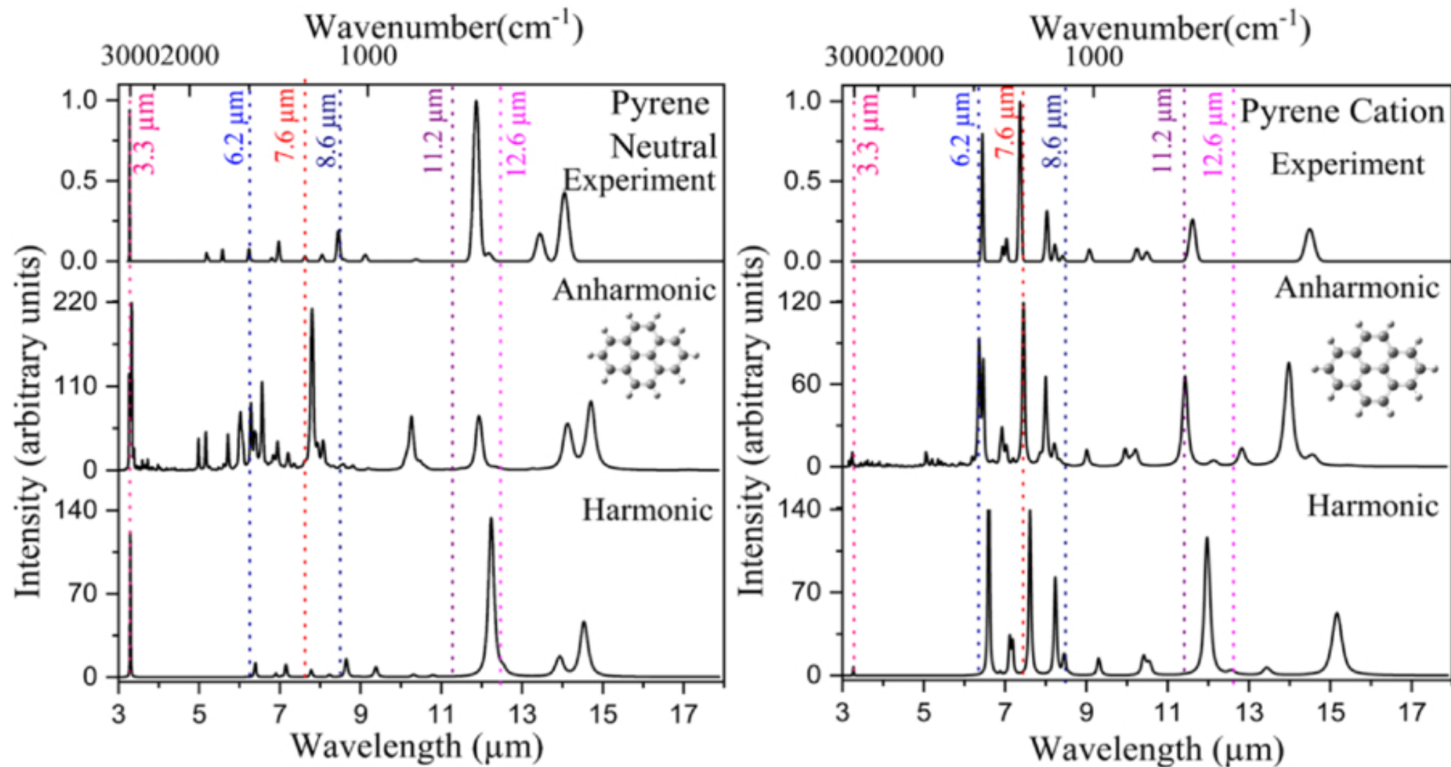
Figure 7. from Venkata Lakshmi Karri et al 2026 Astrophys. J. 1008 doi:10.3847/1538-4357/ae6eef https://dx.doi.org/10.3847/1538-4357/ae6eef © 2026. The Author(s). Published by the American Astronomical Society.
