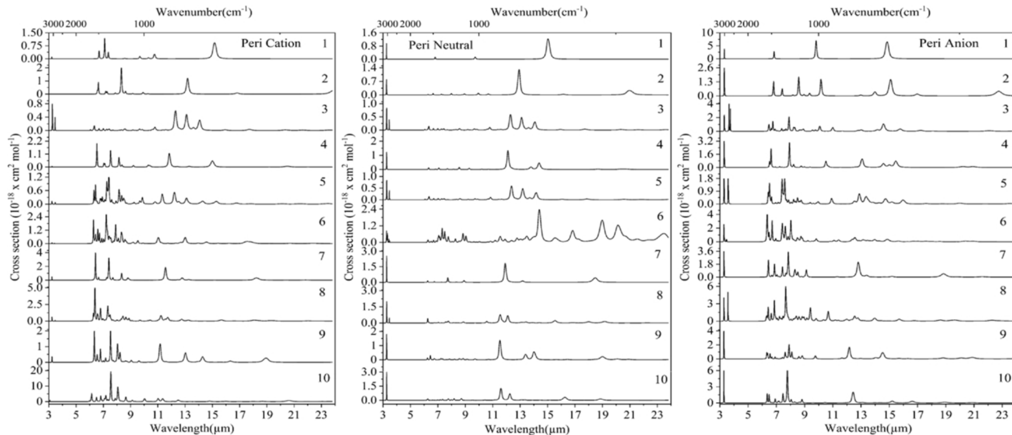
Figure 5. from Venkata Lakshmi Karri et al 2026 Astrophys. J. 1008 doi:10.3847/1538-4357/ae6eef https://dx.doi.org/10.3847/1538-4357/ae6eef © 2026. The Author(s). Published by the American Astronomical Society.
