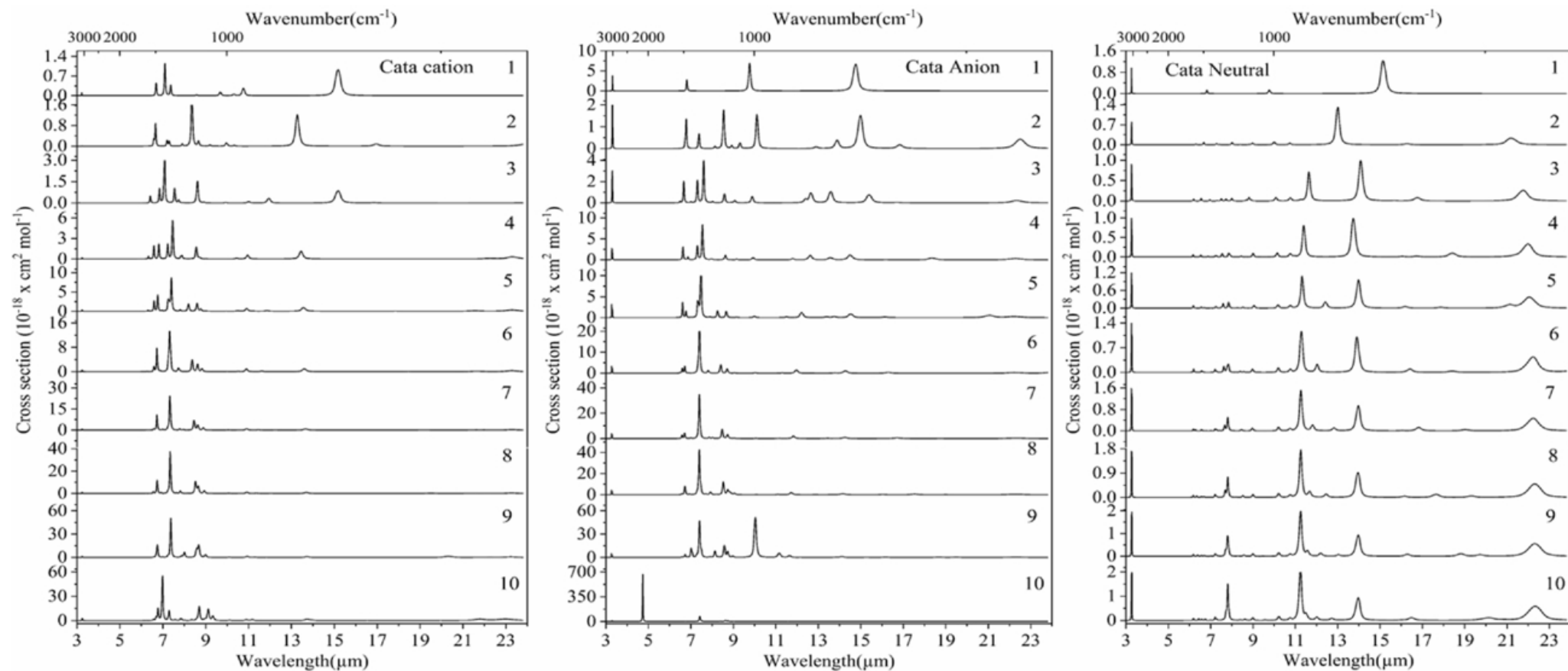
Figure 4. from Venkata Lakshmi Karri et al 2026 Astrophys. J. 1008 doi:10.3847/1538-4357/ae6eef https://dx.doi.org/10.3847/1538-4357/ae6eef © 2026. The Author(s). Published by the American Astronomical Society.
