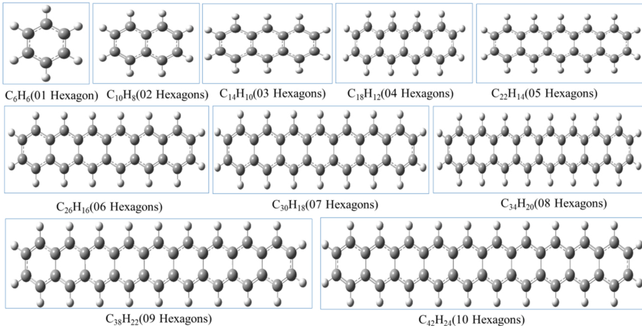
Figure 2. from Venkata Lakshmi Karri et al 2026 Astrophys. J. 1008 doi:10.3847/1538-4357/ae6eef https://dx.doi.org/10.3847/1538-4357/ae6eef © 2026. The Author(s). Published by the American Astronomical Society.
