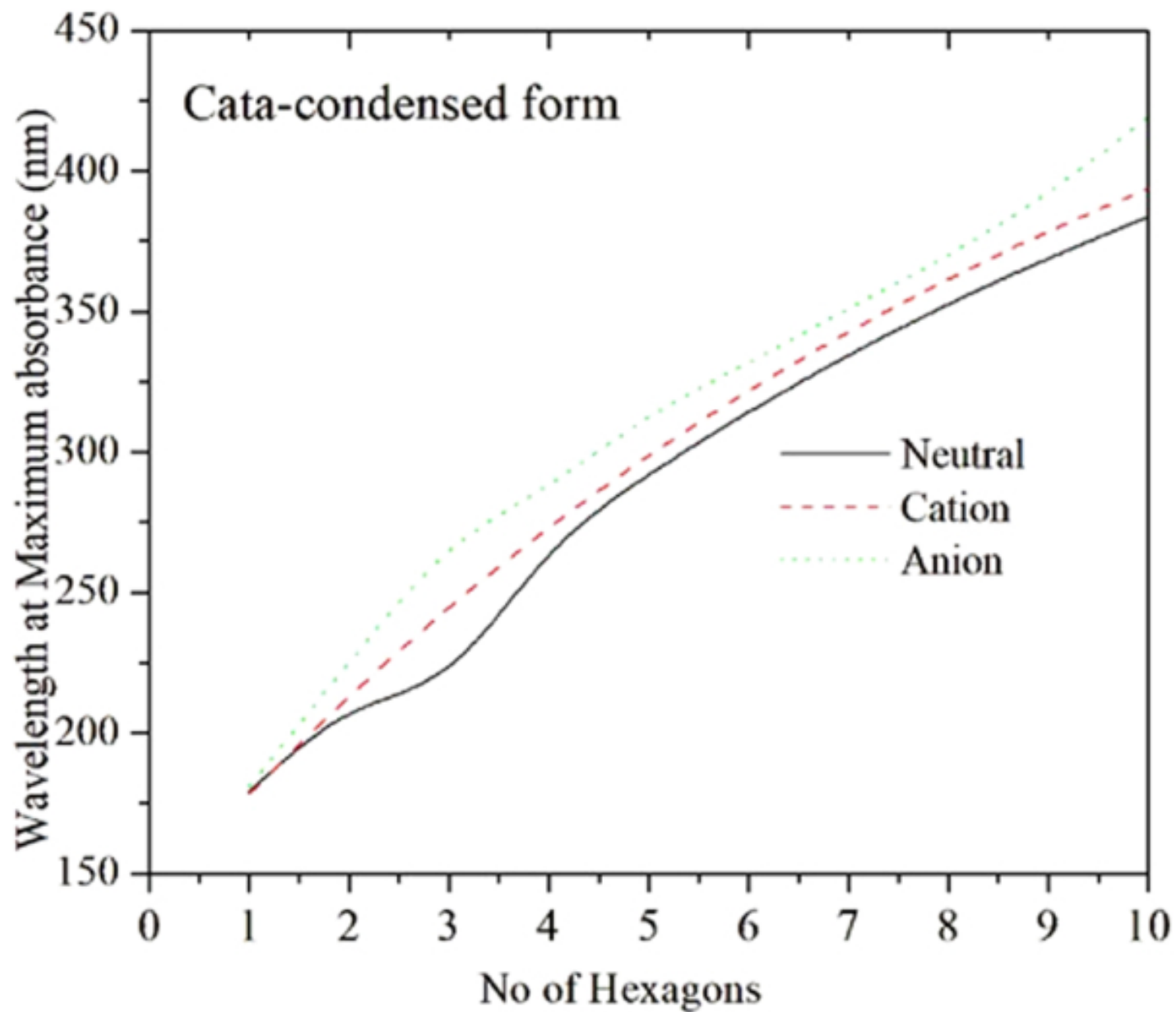
Figure 16. from Venkata Lakshmi Karri et al 2026 Astrophys. J. 1008 doi:10.3847/1538-4357/ae6eef https://dx.doi.org/10.3847/1538-4357/ae6eef © 2026. The Author(s). Published by the American Astronomical Society.
