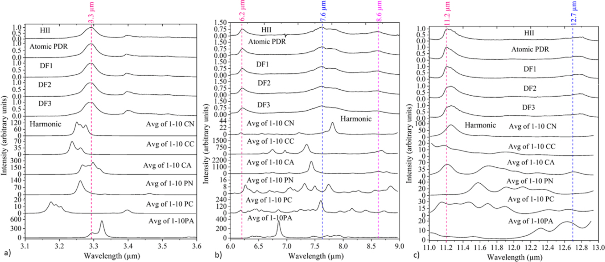
Figure 14. from Venkata Lakshmi Karri et al 2026 Astrophys. J. 1008 doi:10.3847/1538-4357/ae6eef https://dx.doi.org/10.3847/1538-4357/ae6eef © 2026. The Author(s). Published by the American Astronomical Society.
