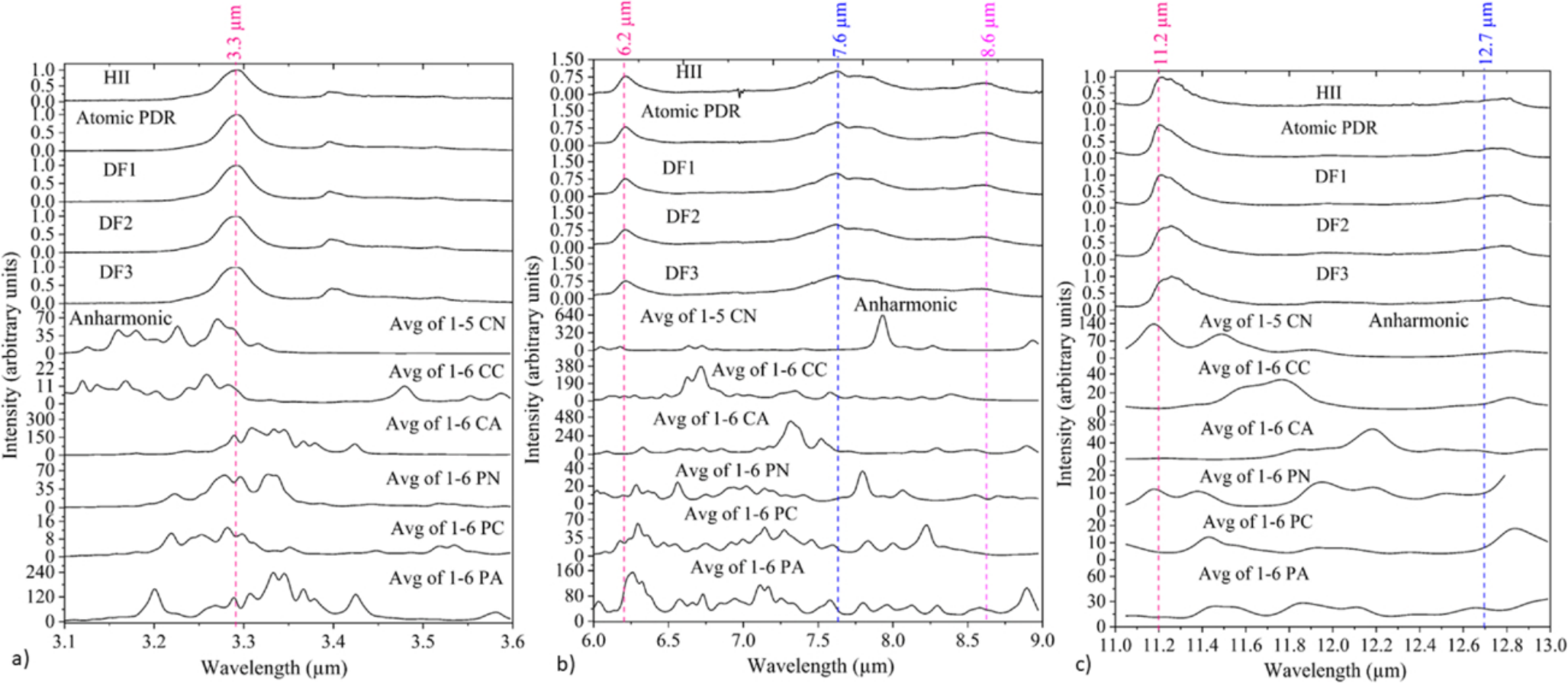
Figure 13. from Venkata Lakshmi Karri et al 2026 Astrophys. J. 1008 doi:10.3847/1538-4357/ae6eef https://dx.doi.org/10.3847/1538-4357/ae6eef © 2026. The Author(s). Published by the American Astronomical Society.
