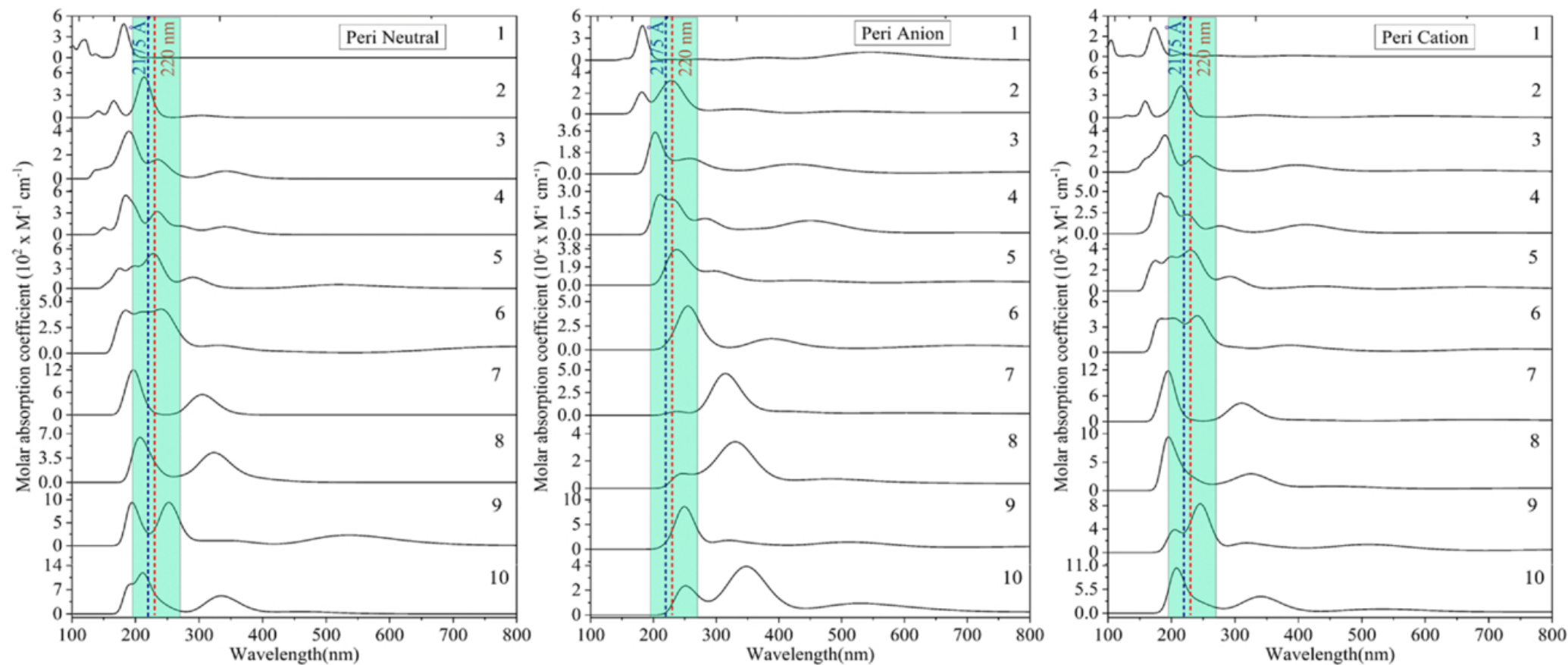
Figure 10. from Venkata Lakshmi Karri et al 2026 Astrophys. J. 1008 doi:10.3847/1538-4357/ae6eef https://dx.doi.org/10.3847/1538-4357/ae6eef © 2026. The Author(s). Published by the American Astronomical Society.
