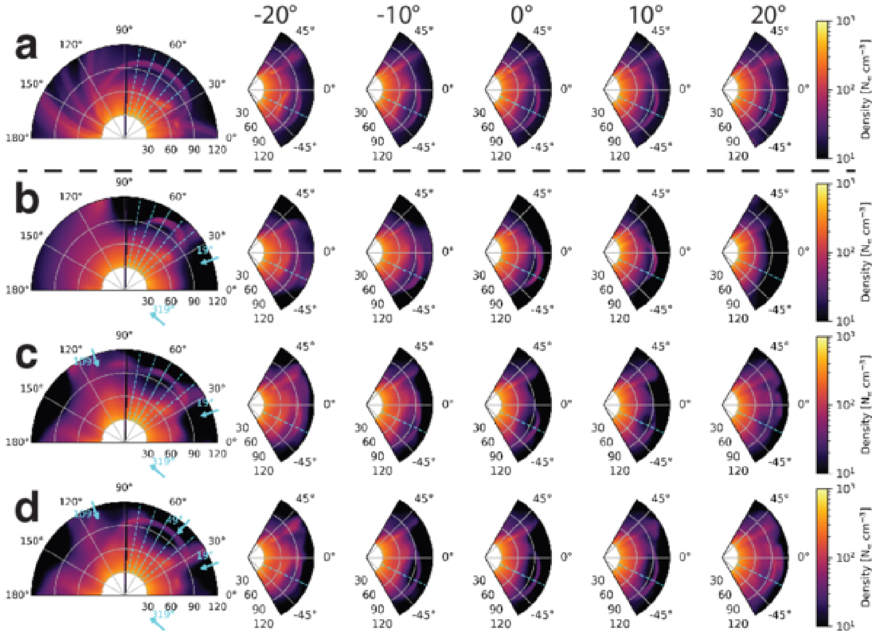
Figure 9. from Robert Jarolim et al 2026 Astrophys. J. 1004 doi:10.3847/1538-4357/ae6e39 https://dx.doi.org/10.3847/1538-4357/ae6e39 © 2026. The Author(s). Published by the American Astronomical Society.
