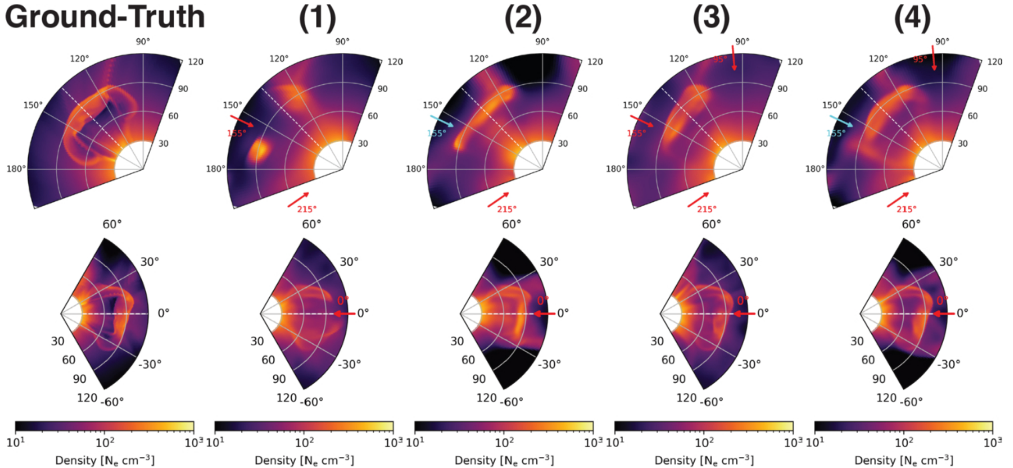
Figure 7. from Robert Jarolim et al 2026 Astrophys. J. 1004 doi:10.3847/1538-4357/ae6e39 https://dx.doi.org/10.3847/1538-4357/ae6e39 © 2026. The Author(s). Published by the American Astronomical Society.
