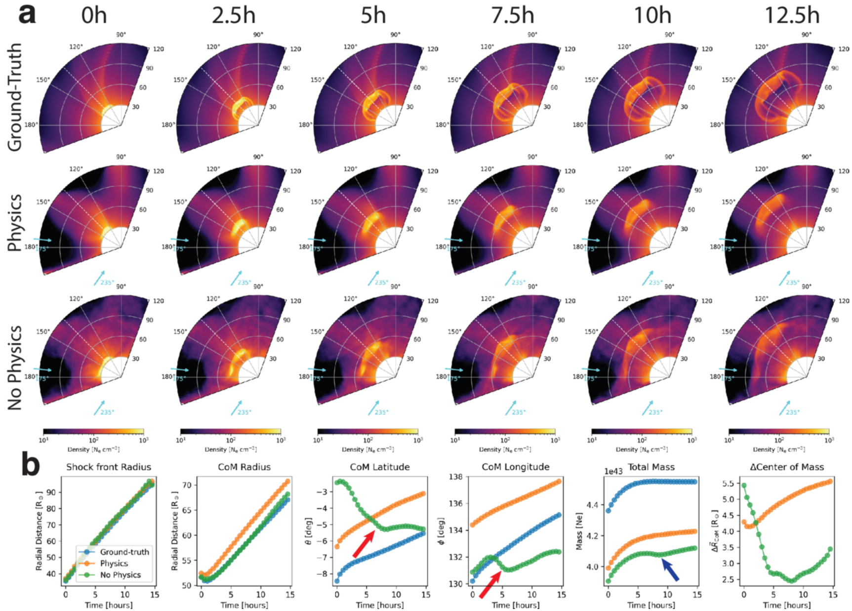
Figure 6. from Robert Jarolim et al 2026 Astrophys. J. 1004 doi:10.3847/1538-4357/ae6e39 https://dx.doi.org/10.3847/1538-4357/ae6e39 © 2026. The Author(s). Published by the American Astronomical Society.
