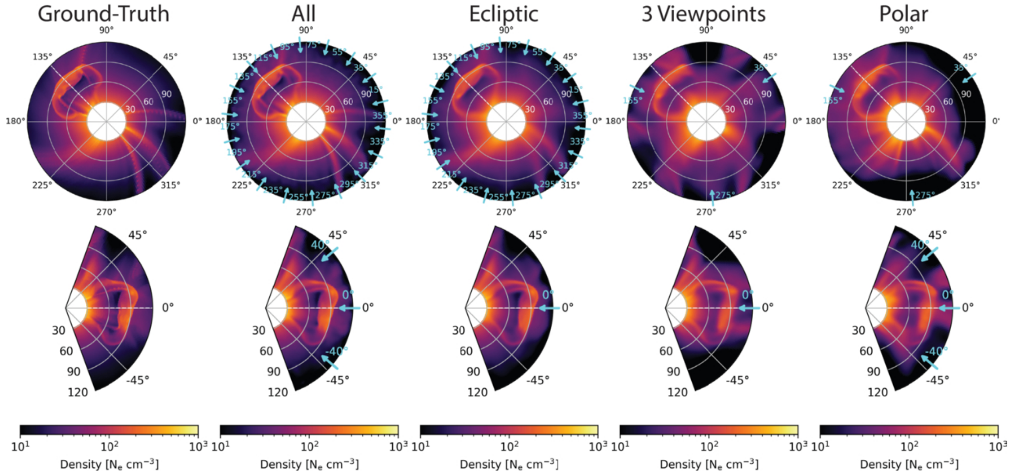
Figure 3. from Robert Jarolim et al 2026 Astrophys. J. 1004 doi:10.3847/1538-4357/ae6e39 https://dx.doi.org/10.3847/1538-4357/ae6e39 © 2026. The Author(s). Published by the American Astronomical Society.
