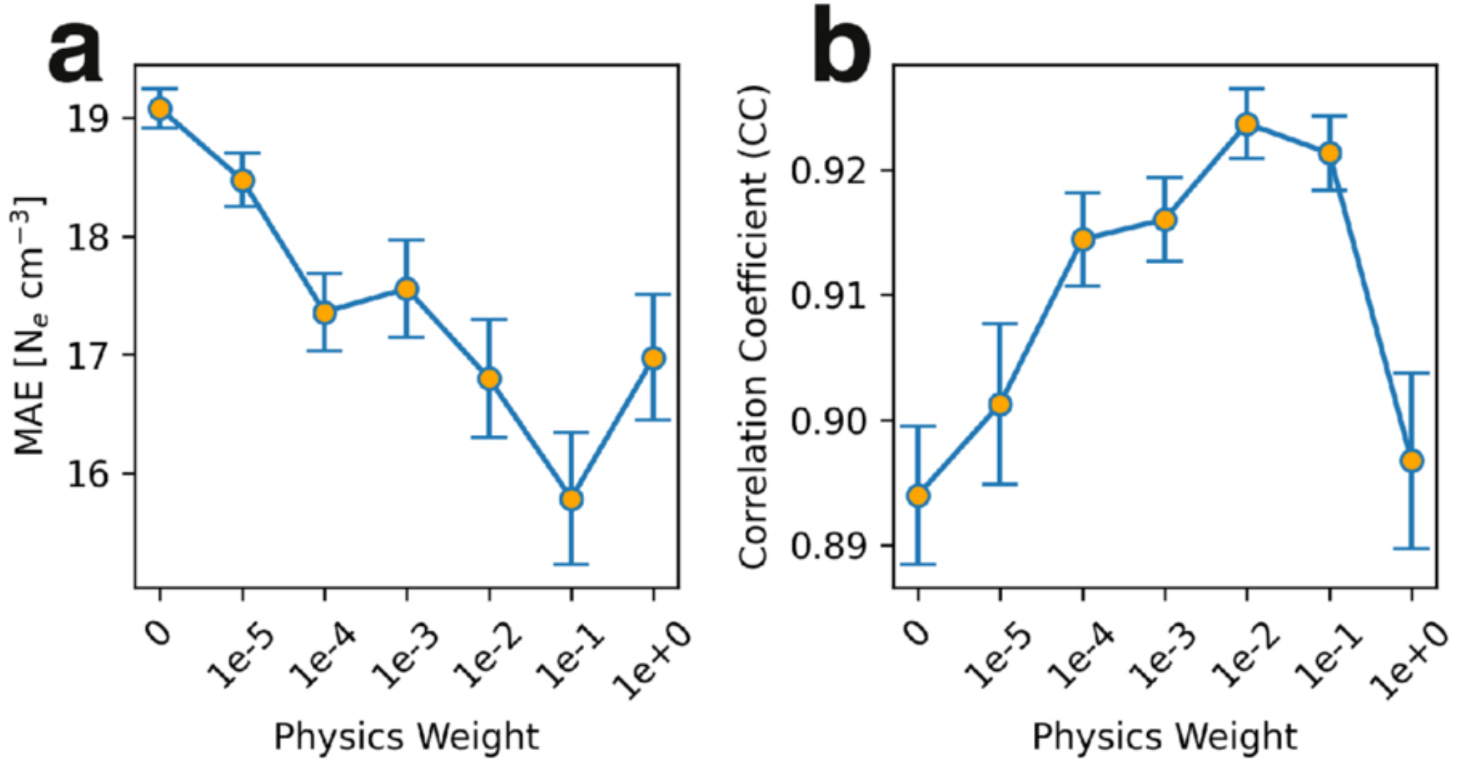
Figure 11. from Robert Jarolim et al 2026 Astrophys. J. 1004 doi:10.3847/1538-4357/ae6e39 https://dx.doi.org/10.3847/1538-4357/ae6e39 © 2026. The Author(s). Published by the American Astronomical Society.
