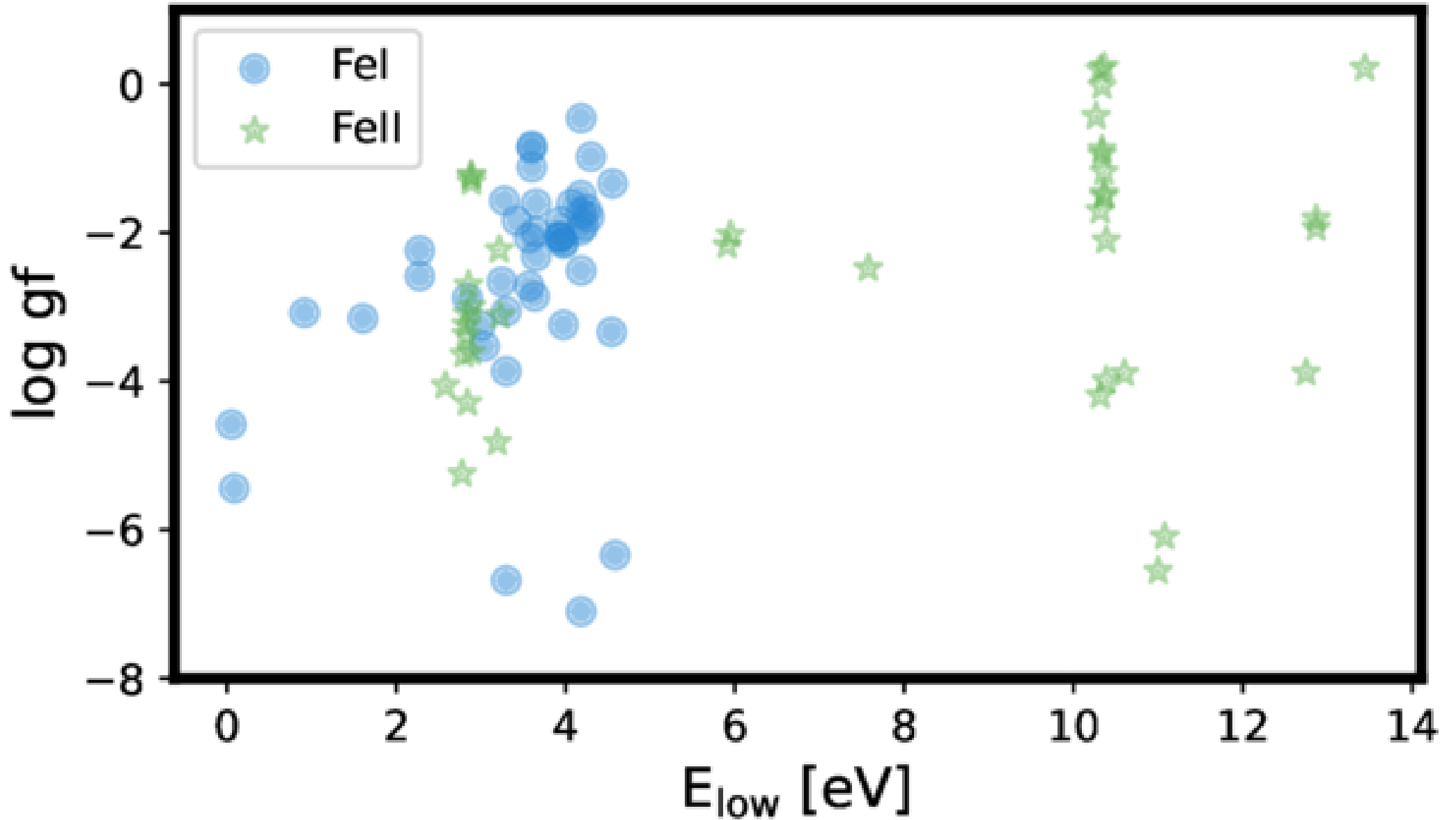
Figure 2. from V. Vasilyev et al 2026 Astrophys. J. 1004 doi:10.3847/1538-4357/ae6e33 https://dx.doi.org/10.3847/1538-4357/ae6e33 © 2026. The Author(s). Published by the American Astronomical Society.
