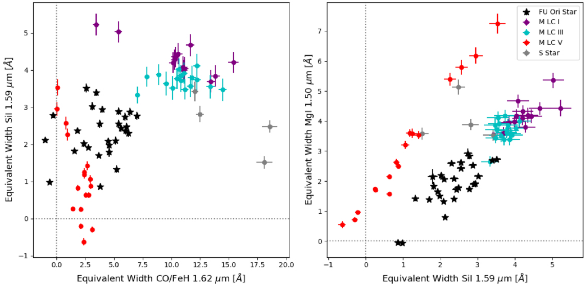
Figure 8. from Evan R. Portnoi et al 2026 Astrophys. J. 1005 doi:10.3847/1538-4357/ae6dbc https://dx.doi.org/10.3847/1538-4357/ae6dbc © 2026. The Author(s). Published by the American Astronomical Society.
