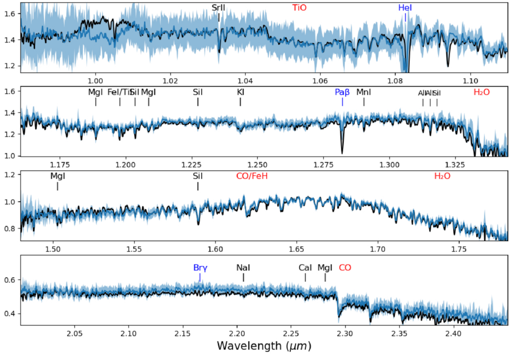
Figure 5. from Evan R. Portnoi et al 2026 Astrophys. J. 1005 doi:10.3847/1538-4357/ae6dbc https://dx.doi.org/10.3847/1538-4357/ae6dbc © 2026. The Author(s). Published by the American Astronomical Society.
