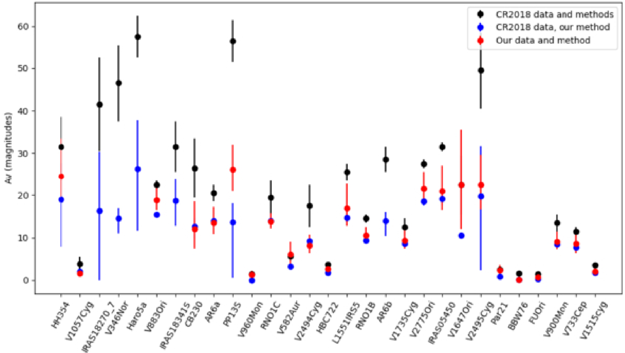
Figure 4. from Evan R. Portnoi et al 2026 Astrophys. J. 1005 doi:10.3847/1538-4357/ae6dbc https://dx.doi.org/10.3847/1538-4357/ae6dbc © 2026. The Author(s). Published by the American Astronomical Society.
